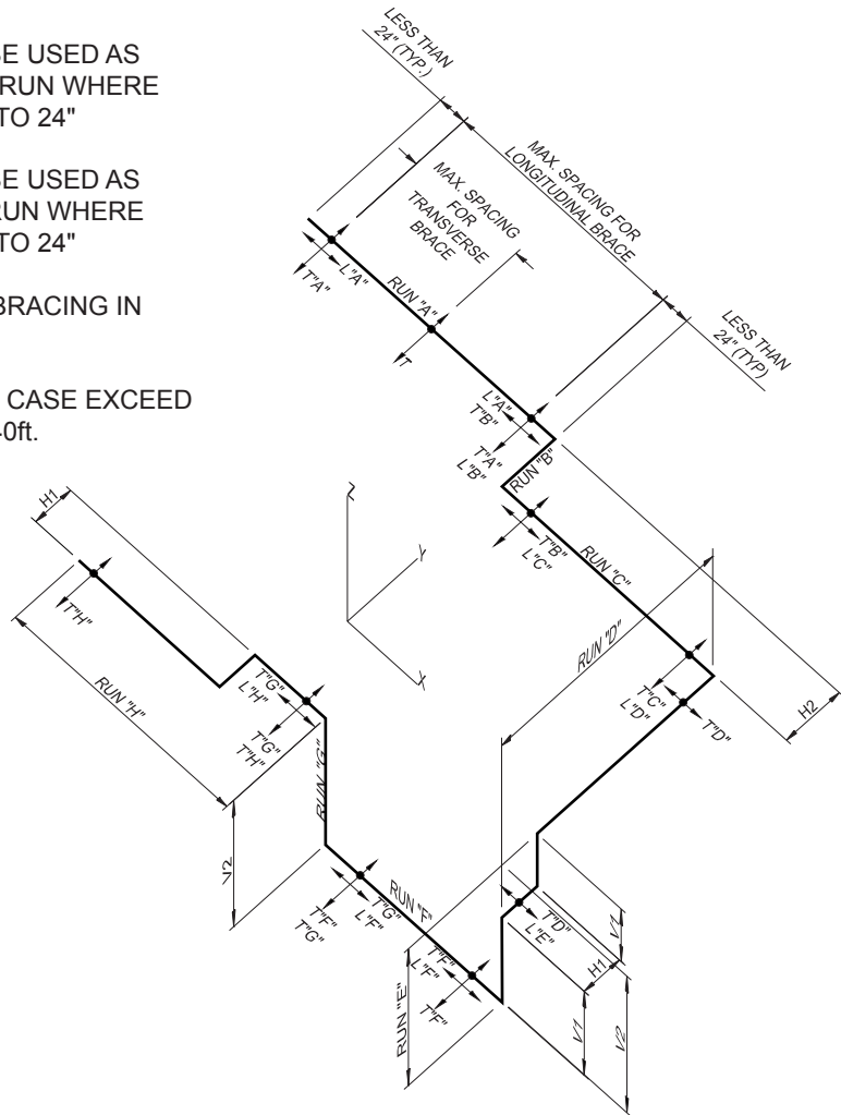
ISOMETRIC DIAGRAM OF TRANSVERESE AND LONGITUDINAL BRACE LOCATION REQUIREMENT
